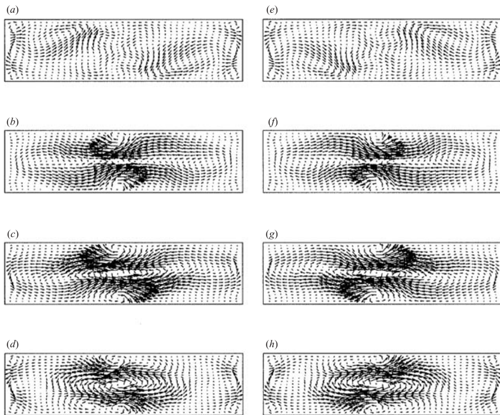
FIGURE 12. Fluctuating velocity field projected onto the H_l plane, and viewed from above: (a) t = 0 , (b) t = T/8 , (c) t = T/4 , (d) t = 3T/8 , (e) t = T/2 , (f) t = 5T/8 , (g) t = 3T/4 , (h) t = 7T/8 . The parameters are Gr = 49\,000 , Pr = 0.019 .
